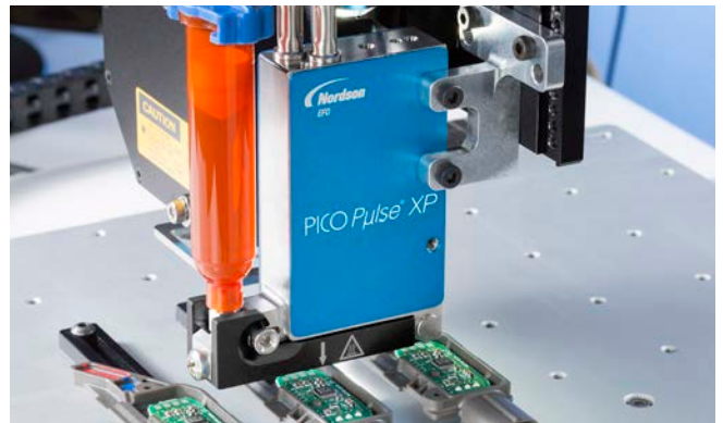
PICO Pulse XP's sustained stroke target seeking maintains long-term dispensing repeatability.
